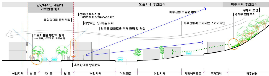
B-B' Section
